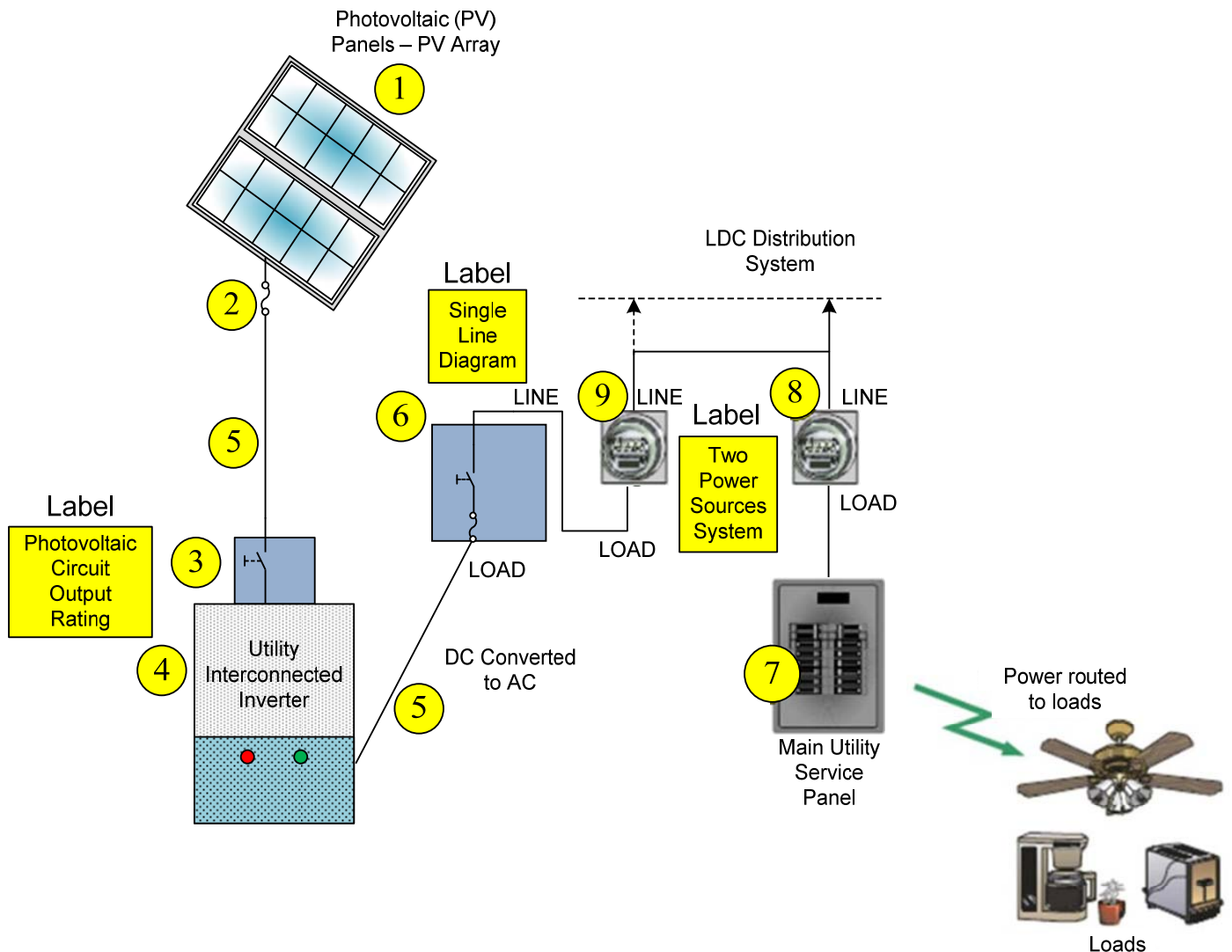
Diagram B: Parallel Meter Connection – microFIT Project
